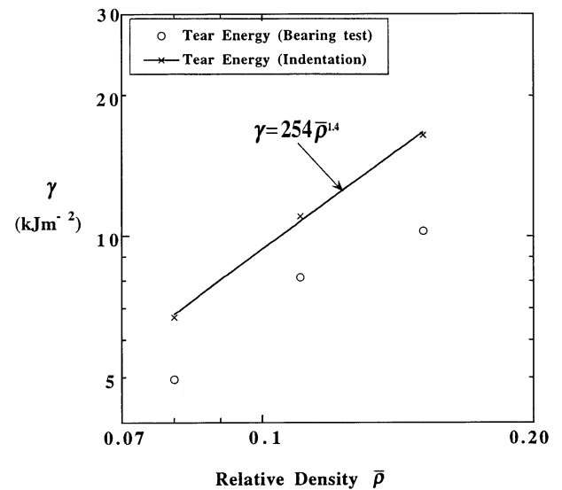
Figure 15 Tear energies for Alporas metallic foams of different relative density. Tear energies determined from bearing and deep-indentation tests.
