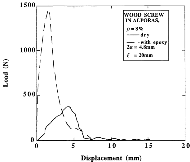
Figure 2 Load-displacement curves for both dry and epoxy-bonded wood screws, in Alporas with relative density \bar{\rho} = 8\% . Diameter 2a = 4.8 mm, embedded length \ell = 20 mm.
