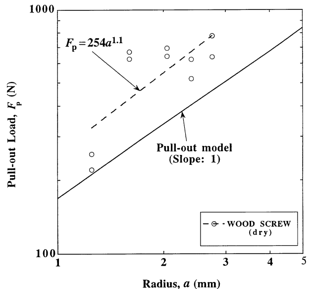
Figure 5 Effect of radius of wood screw (dry), of embedded length \ell = 35 mm, on the pull-out load from Alporas metallic foam, relative density \bar{\rho} = 8\% .
