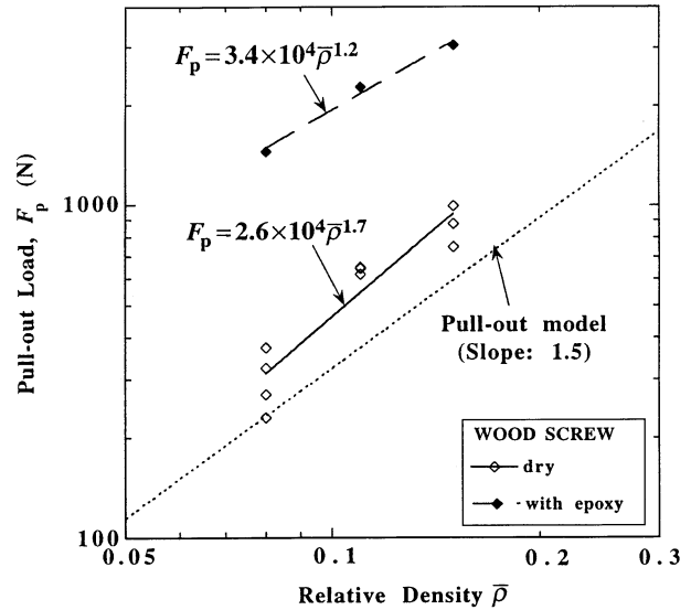
Figure 4 Effect of relative density on pull-out load of wood screw (diameter 2a = 4.8 mm, embedded length \ell = 20 mm), from Alporas metallic foams—comparison of experimental and predicted results. (Open symbols: dry; full symbols: epoxy-bonded).
