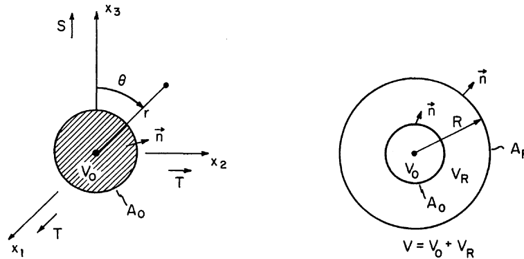
FIG. 2. Geometry and conventions for isolated void calculations.
