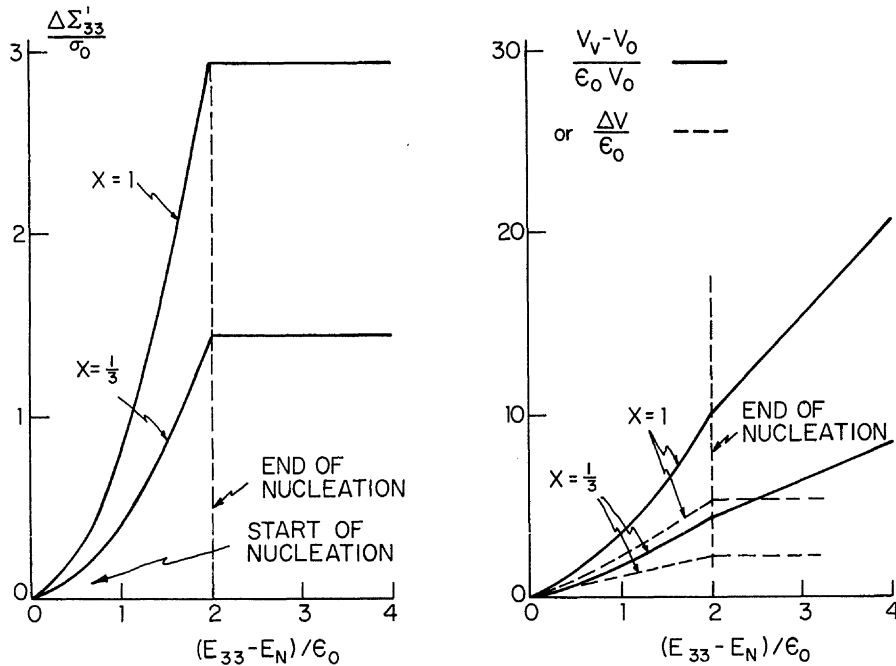
FIG. 3. Stress drop history and volume increase for nucleation and initial growth of a void from a rigid spherical particle of unit volume ( X = 1/3 and 1 , \delta E_N = 2\varepsilon_0 ).
