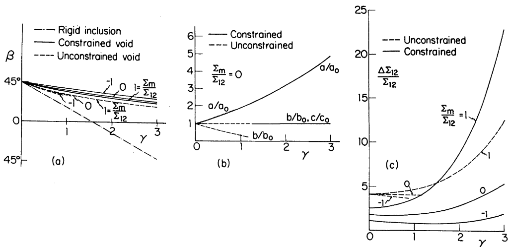
FIG. 16. Evolution with \gamma for a void nucleated as a sphere at \gamma = 0 . (a) Orientation of major axis. (b) Major and minor axes. (c) Shear stress drop for void with unit volume at \gamma = 0 .
