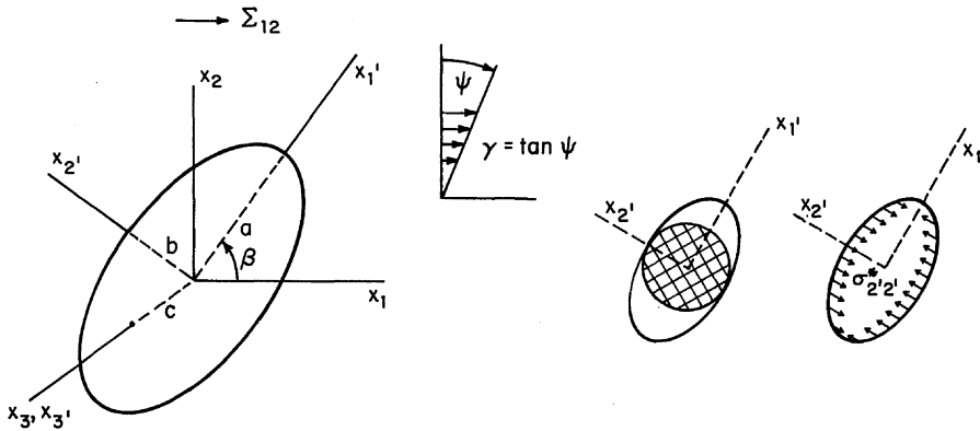
FIG. 15. Geometry for ellipsoidal voids in simple shear.
