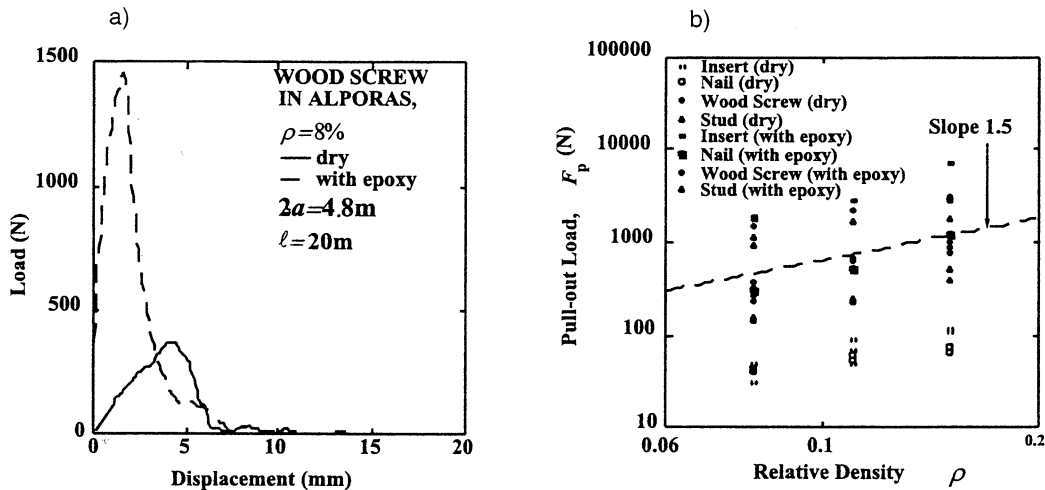
Fig. 2. a) Load-displacement curves for both dry and epoxy-bonded wood screws, in Alporas foam with relative density \rho = 8\% . Diameter 2a = 4.8 mm, embedded length l = 20 mm. b) Dependence of relative density on pull-out load for fasteners. Physical dimension of fasteners are: i) wood screw, diameter 2a = 4.8 mm, embedded length l = 20 mm; ii) nail, diameter 2a = 4.5 mm, embedded length l = 20 mm; iii) stud, diameter 2a = 6 mm, embedded length l = 20 mm; iv) insert, diameter 2a = 20 mm, embedded length l = 20 mm.
