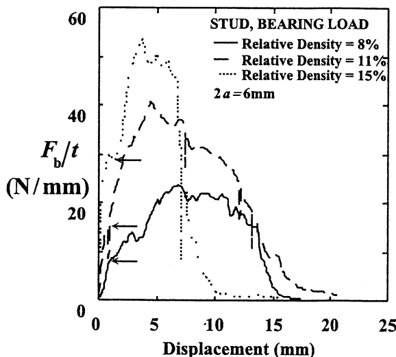
Fig. 3. Pull-through of a 6 mm diameter stud through Alporas metallic foam (specimen dimension 100 \times 40 \times 15 mm), for three densities of foam. The arrows in the figure show initial yield load.
