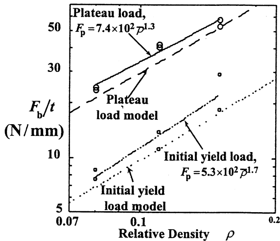
Fig. 4. Plateau bearing load and initial yield load per unit thickness against relative density for Alporas metallic foam, for a 6 mm diameter stud.
