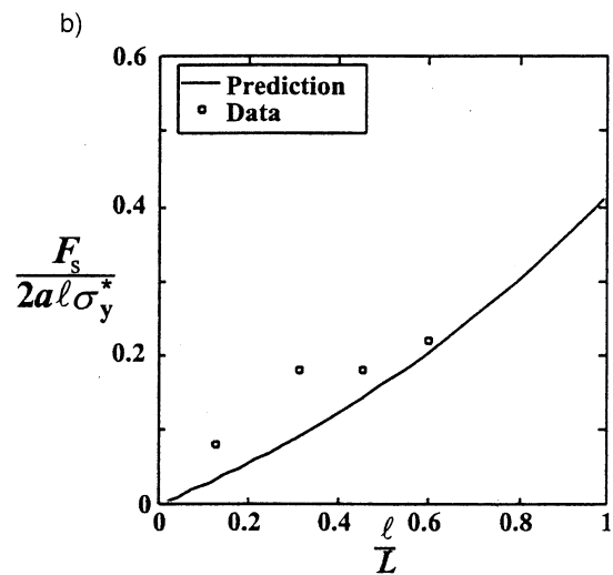
Fig. 6. a) A fastener carrying an end shear load. Rotation occurs about the point X at plastic collapse. b) A comparison of the measured and predicted failure load F_s as a function of the embedded length l . The prediction is given by Equations 10 and 11.
