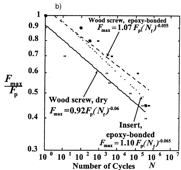
Fig. 5. a) Accumulated displacement under tension-tension cyclic loading of a dry wood screw, diameter 2a = 4.8 mm, embedded length l = 20 mm (Alporas, relative density \rho = 15\% , at R = 0.1 ). Pull-out is progressive with increasing cycles. b) S-N curves for pull-out of fasteners: dry and epoxy-bonded wood screws, and epoxy-bonded insert. Load ratio, R = 0.1 .
