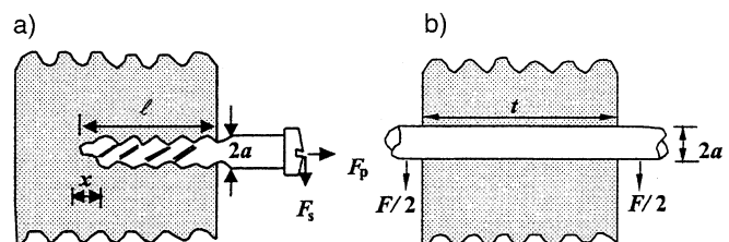
Fig. 1. Typical fastener joints: a) wood screw, b) stud.
