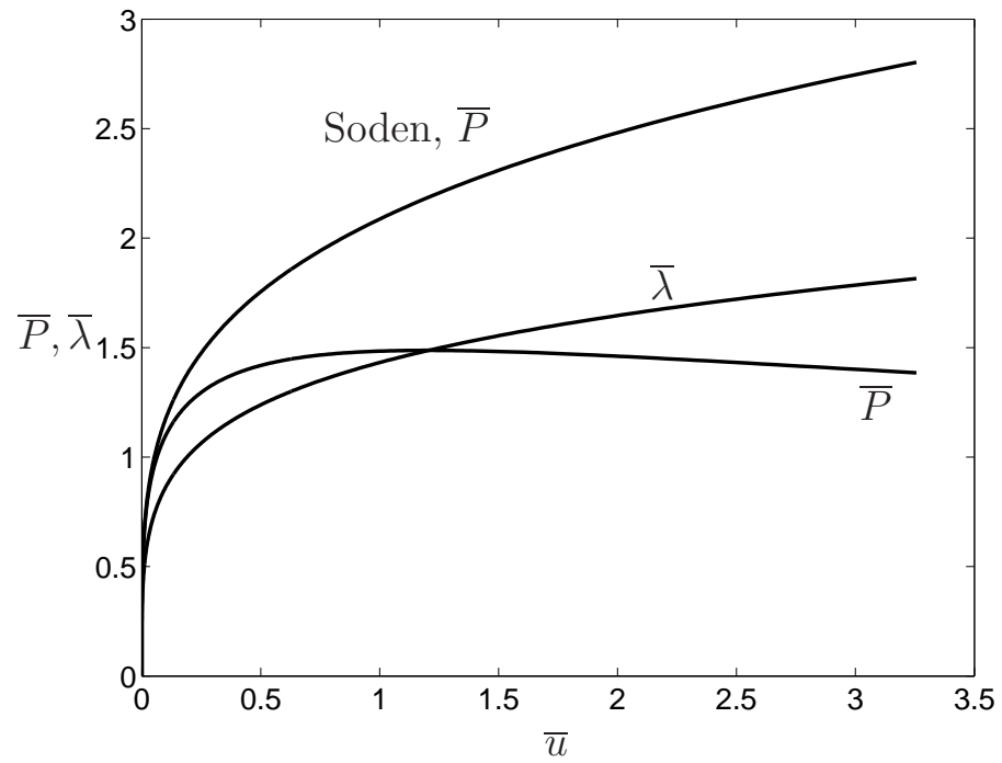
Figure 4: Indentation response of a sandwich beam with a rigid - ideally plastic core. The curves labelled \bar{P} and \bar{\lambda} refer to the indentation response for a sandwich beam in bending, while the curve labelled 'Soden, \bar{P} ' refers to a transversely loaded beam on a half-space.
