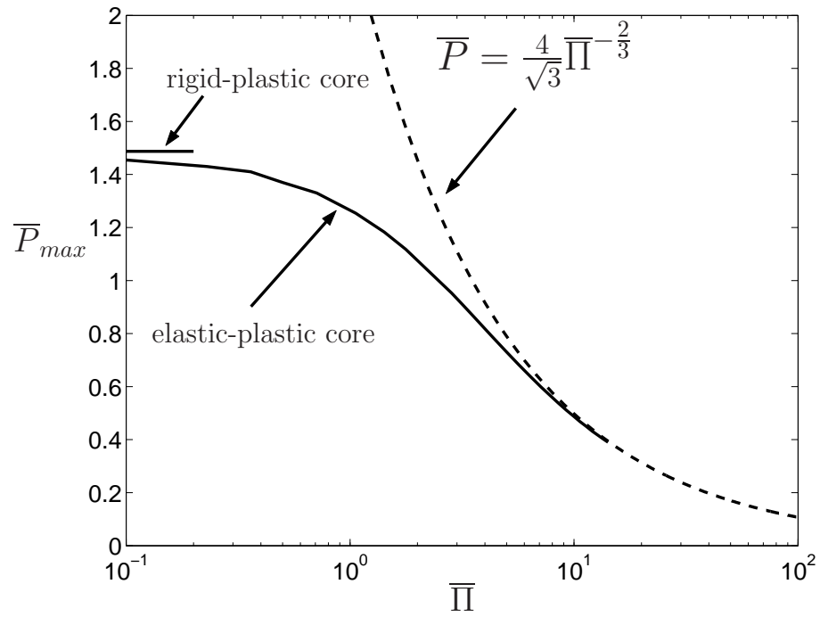
Figure 8: Dependence of the non-dimensional peak load \bar{P}_{max} upon the compliance \bar{\Pi} for the indentation collapse mode. The dotted line refers to the Hetenyi model.
