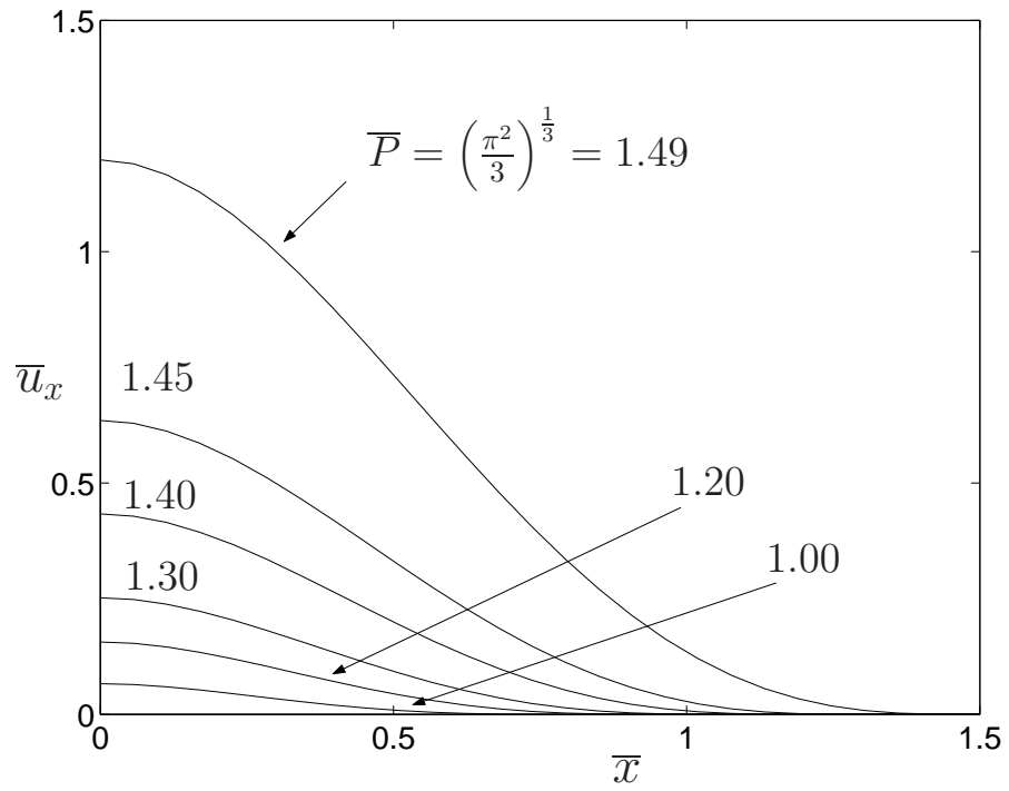
Figure 5: Deflected shape of the compressive face of a sandwich beam with a rigid - ideally plastic core at selected loads up to the peak value \bar{P} = 1.49 .
