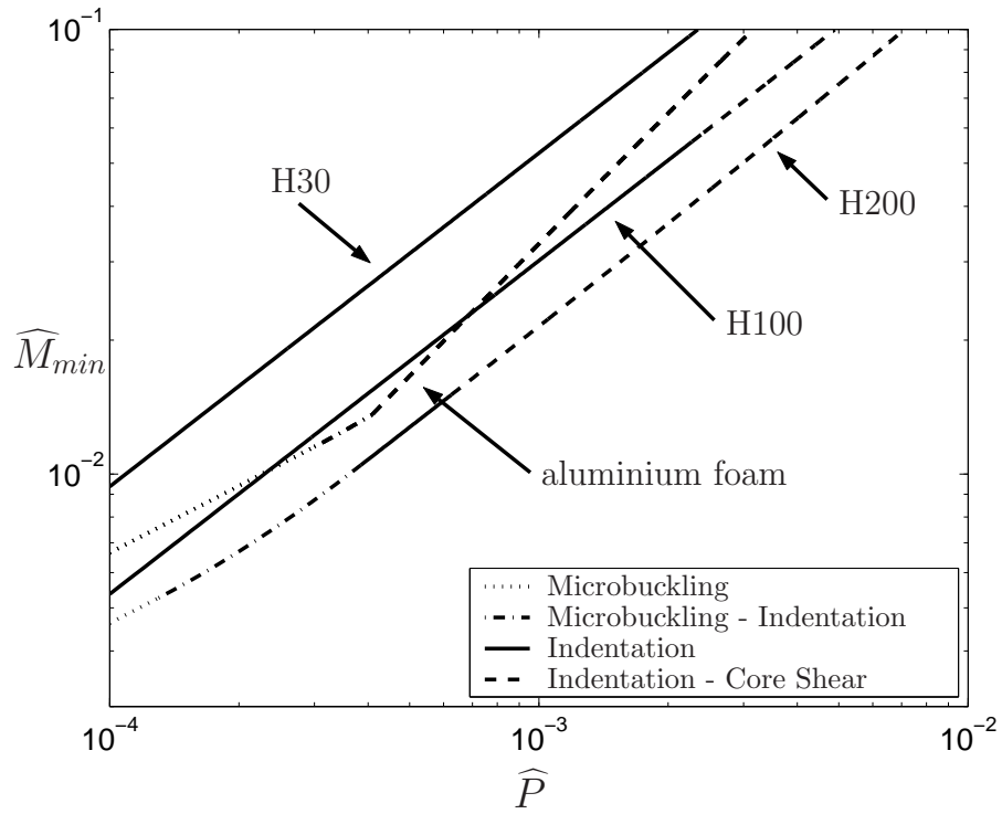
Figure 14: Dependence of the minimum mass \widehat{M}_{min} upon the structural load index \widehat{P} , for composite face sheets and three densities of PVC foam core (H30, H100, and H200), and for an aluminium alloy face sheet and an aluminium alloy foam core. Mass indices for the aluminium sandwich beams are normalised by the density of GFRP.
