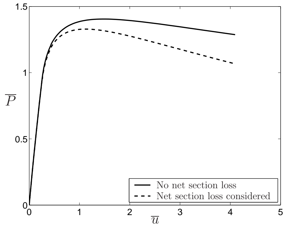
Figure 11: Effect of net section loss upon the indentation response of a sandwich beam with an elastic - ideally plastic core, \bar{\Pi} = 0.36 .
