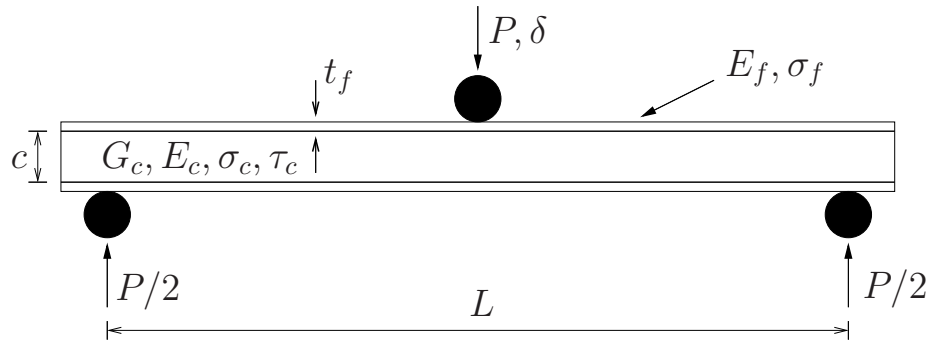
Figure 1: Geometry of sandwich beam.
