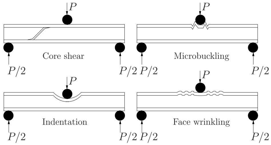
Figure 2: Competing failure modes of sandwich beams subjected to three-point bending.
