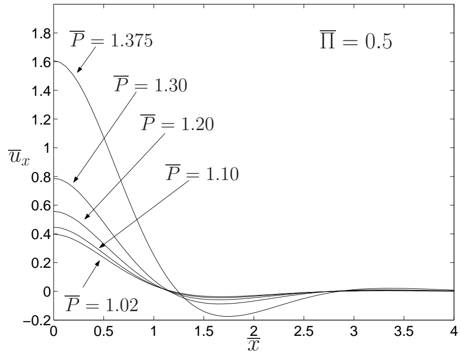
Figure 9: Deflected shape of the compressive face of a sandwich beam with an elastic - ideally plastic core at selected loads up to the peak load; indentation collapse mode.
