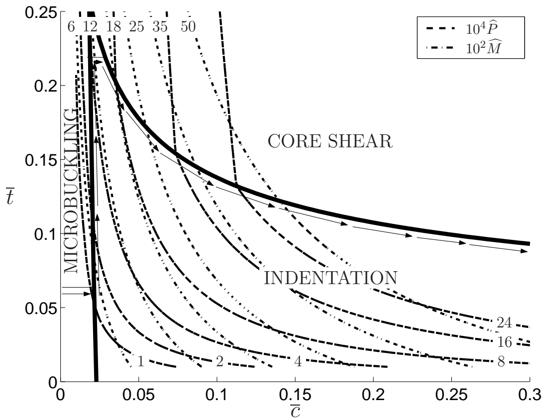
Figure 12: Failure mechanism map of high density H200 foam core with contours of mass index \widehat{M} and structural load index \widehat{P} , and trajectory of minimum weight design. The solid bold lines denote the boundaries between collapse regimes and the arrows follow the minimum weight trajectory.
