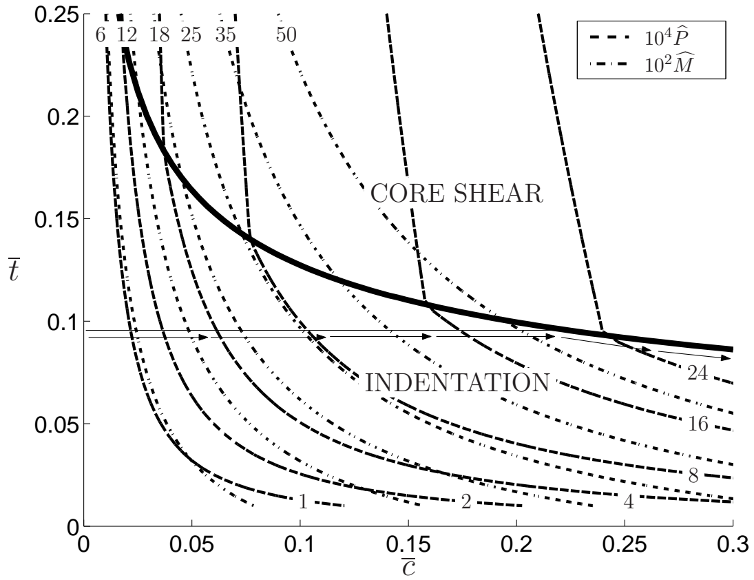
Figure 13: Failure mechanism map for medium density H100 foam core with contours of mass index \widehat{M} and structural load index \widehat{P} . The solid bold line denotes the boundary between the indentation and core shear regimes, and the arrows follow the minimum weight trajectory.
