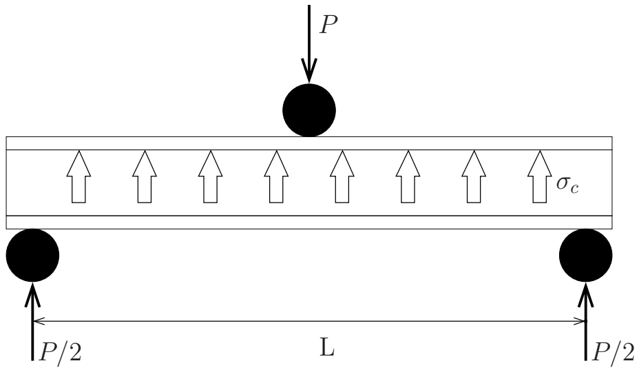
Figure 10: Core crush of a short sandwich beam.
