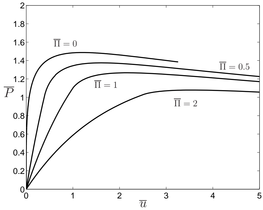
Figure 6: The effect of core compliance, as parameterised by \bar{\Pi} , upon the non-dimensional load versus displacement response for a sandwich beam with an elastic-ideally plastic core; indentation collapse mode.
