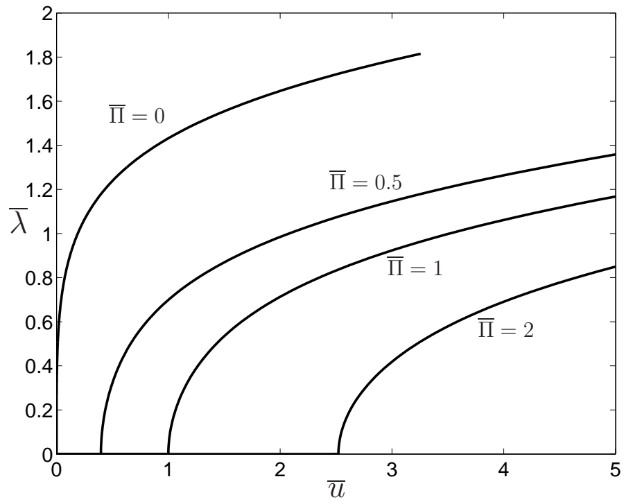
Figure 7: The effect of core compliance, as parameterised by \bar{\Pi} , upon the size of the indentation zone for a sandwich beam with an elastic-ideally plastic core; indentation collapse mode.
