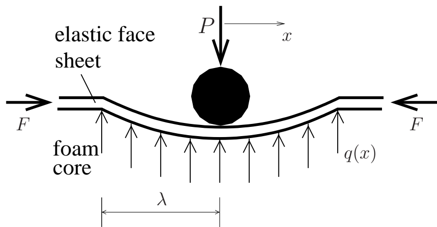
Figure 3: Indentation zone beneath loading roller.
