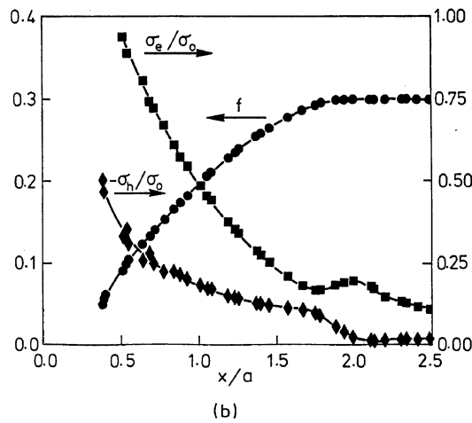
Fig. 16. Variation of normalized macroscopic effective stress, \sigma_e/\sigma_0 , normalized hydrostatic stress, \sigma_h/\sigma_0 , and porosity, f , directly ahead of indenter along the axis of symmetry. (a) Gurson solid, with initial porosity f_0 = 0.1 , (b) FKM solid, with initial porosity f_0 = 0.3 . E_0/\sigma_0 = 500 , \nu_0 = 0.3 , \beta = 19.7^\circ .
