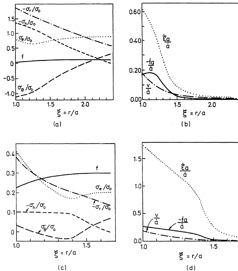
Fig. 6. Predictions of the cavity expansion model. E_0/\sigma_0 = 500 , \nu_0 = 0.3 , \beta = 19.7^\circ . Spatial dependence of (a) stresses and porosity, and (b) rate quantities for the Gurson solid, with initial porosity f_0 = 0.1 . Spatial dependence of (c) stresses and porosity, and (d) rate quantities for the FKM solid, with initial porosity f_0 = 0.3 .
