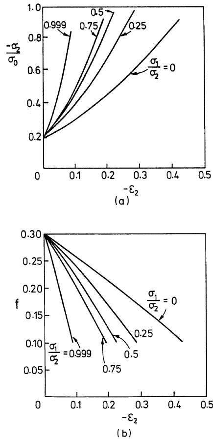
Fig. 4. Response of the FKM solid with initial porosity f_0 = 0.3 to proportional multi-axial compression. E_0/\sigma_0 = 1000 , \nu_0 = 0.3 . (a) True stress versus logarithmic strain. (b) Evolution of porosity.
