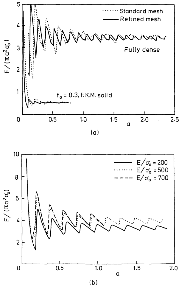
Fig. 10. (a) Effect of mesh refinement upon average indentation pressure, (b) effect of yield strain upon average indentation pressure. \nu_0 = 0.3 , \beta = 19.7^\circ , E/\sigma_0 = 200 unless otherwise stated.
