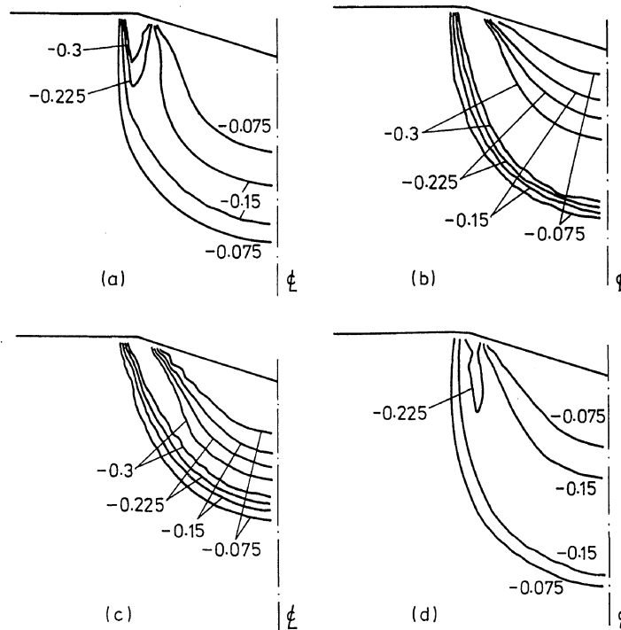
Fig. 15. Contours of constant porosity rate, \dot{f}h/\dot{h} , for (a) Gurson solid, with initial porosity f_0 = 0.1 , (b) FKM solid, with initial porosity f_0 = 0.1 , (c) Gurson solid, with initial porosity f_0 = 0.3 , (d) FKM solid, with initial porosity f_0 = 0.3 . E_0/\sigma_0 = 500 , \nu_0 = 0.3 , \beta = 19.7^\circ .
