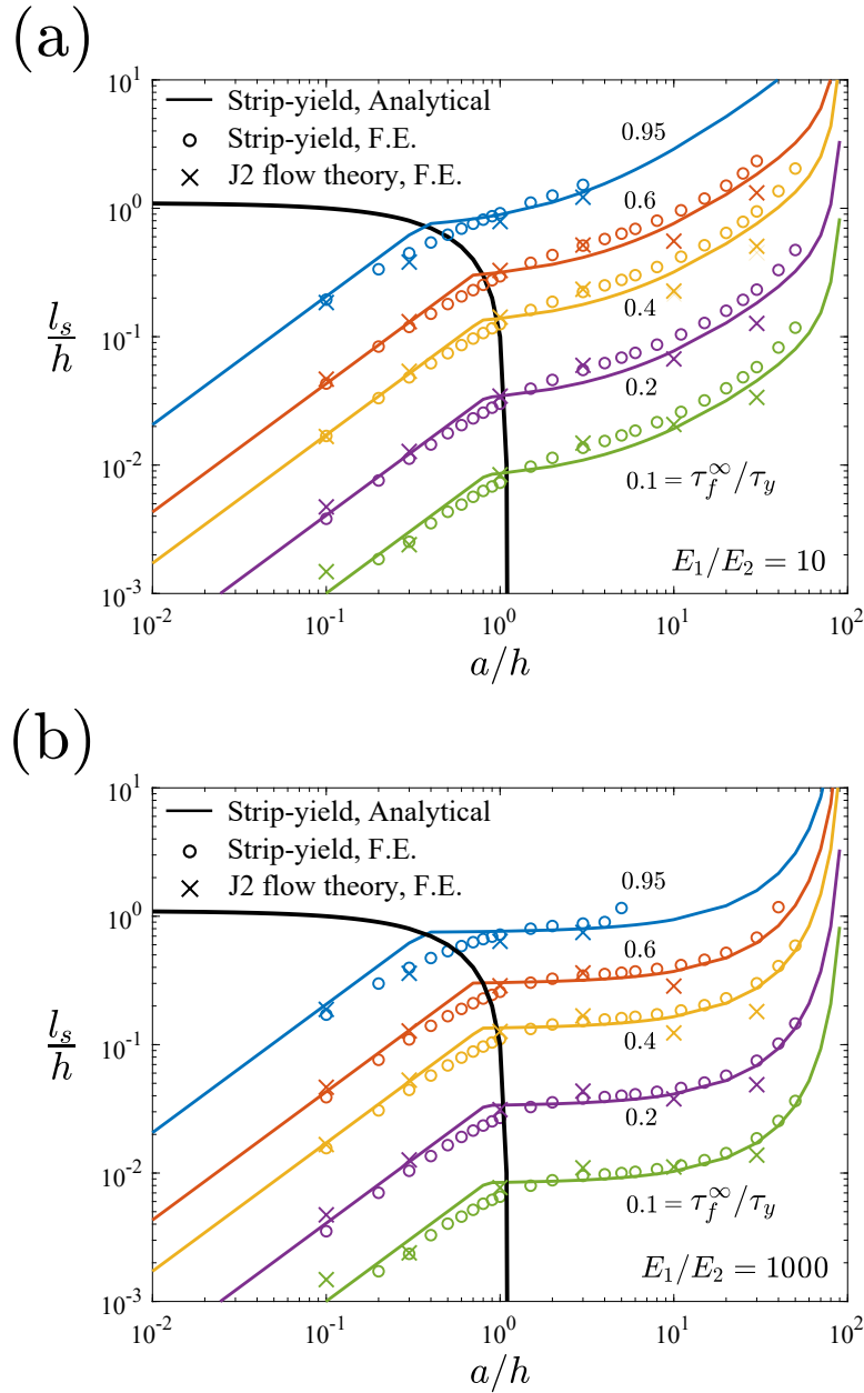
Figure 14: Failure map of l_s/h versus normalized crack length a/h for h/W = 0.01 and mismatch (a) E_1/E_2 = 10 and (b) E_1/E_2 = 1000 . The black solid line separates the regimes A and B from the regimes C and D.
