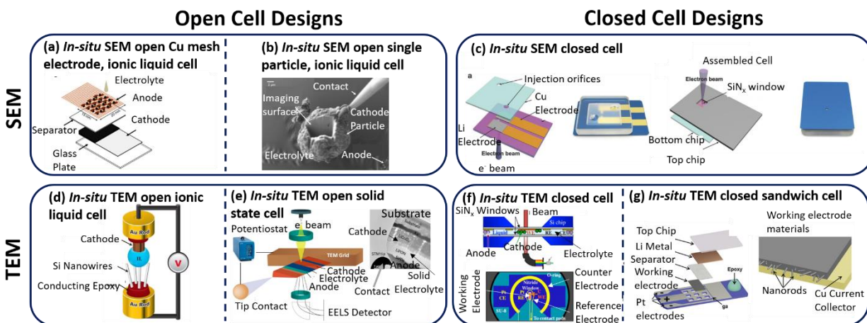
Figure 11. Examples of open and closed cell in-situ TEM and SEM designs. a) Open cell in-situ SEM cell design consisting of active material particles on a copper mesh in a sandwich cell geometry with an ionic liquid electrolyte, reproduced from Ref. 250 [Chen, Sano, Tsuda, Ui, Oshima, Yamagata, Ishikawa, Haruta, Doi, Inaba, and Kuwabata, Scientific Reports (2016)] under Creative Commons Attribution CC BY 4.0. b) open cell in-situ SEM cell with an active material particle cathode suspended on an ionic liquid electrolyte and lithium titanate anode, 263 (Miller, Proff, Wen, Abraham, and Bareño, Advanced Energy Materials) Copyright © 2013 WILEY-VCH Verlag GmbH & Co. KGaA, Weinheim. c) closed cell in-situ SEM design utilising SiN x observation windows, 258 (Rong, Zhang, Zhao, Qiu, Liu, Ye, Xu, Chen, Hou, Li, Duan, and Zhang, Advanced Materials) © 2017 WILEY-VCH Verlag GmbH & Co. KGaA, Weinheim. d) open cell in-situ TEM cell using Si nanowires and an ionic liquid electrolyte, 249 reprinted with permission from (Gu, Parent, Mehdi, Unocic, McDowell, Sacci, Xu, Connell, Xu, Abellan, Chen, Zhang, Perea, Evans, Lauhon, Zhang, Liu, Browning, Cui, Arslan, and Wang, Nano Letters 13, 6106). Copyright (2013) American Chemical Society. e) open all solid state cell in-situ TEM cell created using a FIB sectioning, 254 reprinted with permission from (Wang, Santhanagopalan, Zhang, Wang, Xin, He, Li, Dudney, and Meng, Nano Letters 16, 3760). Copyright (2016) American Chemical Society. f) closed cell in-situ TEM cell in a 3-electrode configuration using an organic liquid electrolyte, 257 reprinted with permission from (Holtz, Yu, Gunceler, Gao, Sundararaman, Schwarz, Arias, Abruña, and Muller, Nano Letters 14, 1453). Copyright (2014) American Chemical Society. g) closed cell in-situ TEM cell in a sandwich geometry with a Li metal anode. 260 (Xu, Zhang, Liu, Li, Zhao, Li, Zhang, and Zhang, Small) © 2020 WILEY-VCH Verlag GmbH & Co. KGaA, Weinheim.
