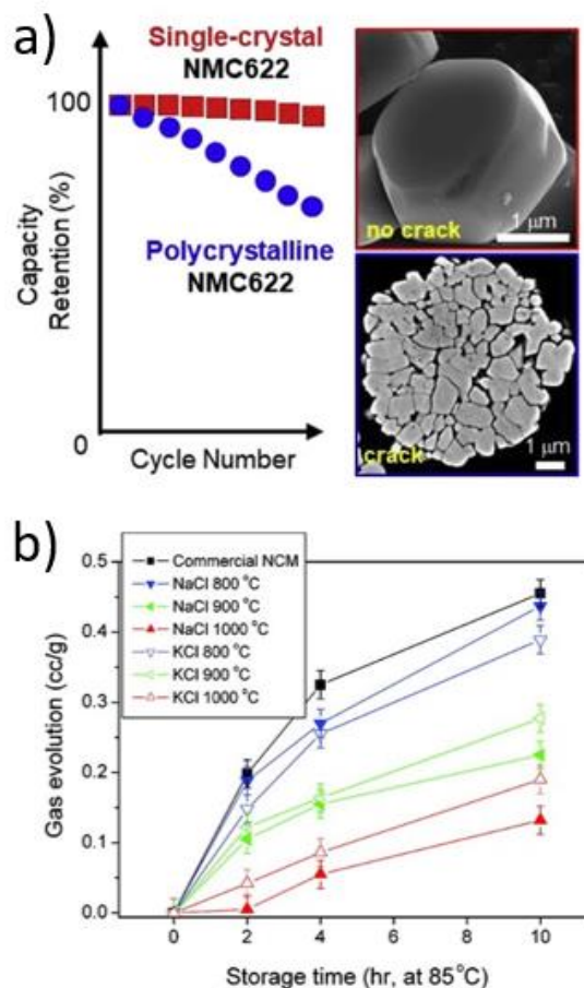
Figure 3. a) Cyclic performance and SEM image of single crystal and polycrystalline NMC cathodes after 300 cycles. Reprinted from Energy Storage Materials , Vol 27, Qian, Zhang, Li, Zhang, Xu, Cheng, Xie, Wang, Rao, He, Shen, Chen, Tang, Ma, Single-crystal nickel-rich layered-oxide battery cathode materials: synthesis, electrochemistry, and intra-granular fracture, 140-149, Copyright (2020), with permission from Elsevier. b) Evolution of gas (cc/gram of NCM) from charged electrodes (4.45 V) with respect to storage time at 85 °C. Reprinted with permission from (Y. Kim, ACS Applied Materials & Interfaces 4, 2329. Copyright (2012) American Chemical Society.
