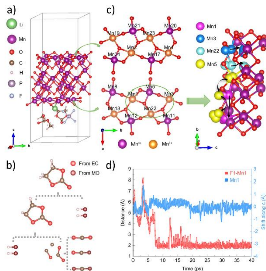
Figure 18. The dissolution processes of Mn in Mn oxides based on AIMD. a) The cathode–electrolyte interface model includes Mn oxide’s (110) slab and electrolytes (EC, DMC, and LiPF 6 ). b) The stepwise oxidative decomposition process of EC molecules. c) Mn ions with different valence states at the interface layer. Synergistic movement of Mn 4+ (Mn5) and its surrounding Mn 3+ (Mn1, Mn3, and Mn22). (d) Interaction between F - from LiPF 6 and surface Mn ion. F - has negligible effect on Mn dissolution. Reprinted with permission from {G. Zhou, X. Sun, Q.H. Li, X. Wang, J.N. Zhang, W. Yang, X. Yu, R. Xiao, and H. Li, J. Phys. Chem. Lett. 11 , 3051 (2020)}. Copyright {2020} American Chemical Society.
