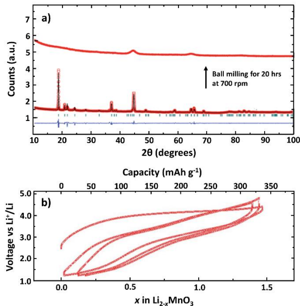
Figure 7. a) The powder X-ray diffraction pattern obtained for \text{Li}_2\text{MnO}_3 as prepared by the solid state reaction after 20 hours of highly energetic ball milling. b) Galvanostatic charge/discharge data obtained for \text{Li}_2\text{MnO}_3 at a rate of 1 \text{Li}^+ per formula unit in 20 hours ( 11.5 \text{ mAh g}^{-1} ) cycling to 4.4 V, 4.6 V and 4.8 V on the first 3 cycles. Reproduced from Ref. 119 from The Royal Society of Chemistry under Creative Commons Attribution CC BY 4.0.
