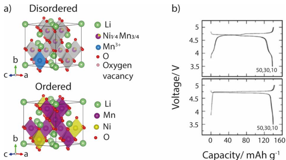
Figure 5. a) Schematic structures of ordered and disordered LNMO materials. b) Charge/discharge curves of disordered (top) and ordered (bottom) LNMO at C/7 (20 mA g -1 ). Figure b) is reprinted with permission from (J.-H. Kim, S.-T. Myung, C.S. Yoon, S.G. Kang, and Y.-K. Sun, Chemistry of Materials 16, 906. Copyright (2004) American Chemical Society).
