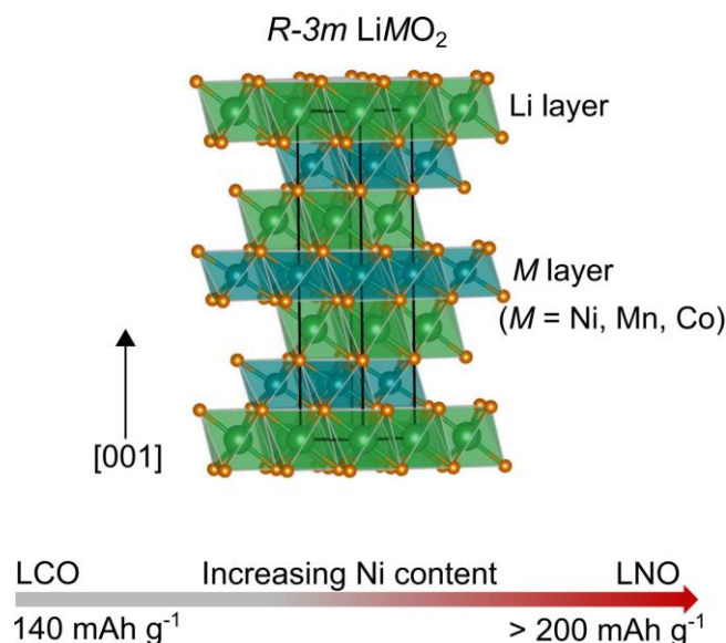
Figure 2. Crystal structure representation of R\text{-}3m \text{LiMO}_2 layered oxide ( M = \text{Ni}, \text{Co}, \text{Mn} ) showing the arrangement of Li and transition metal cations across separate layers. The specific capacities (at practical working potentials) improve upon increasing the Ni content.
