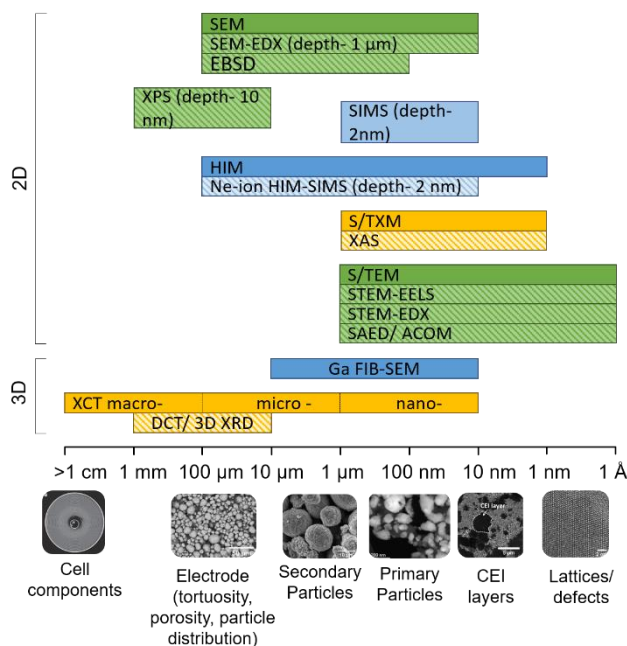
Figure 10. Lateral resolution of different electron (green), ion beam (blue), and X-ray microscopy (yellow) techniques compared with standard cathode morphology components. 238,239 Solid colours represent microscopy techniques, with striped colours representing the associated chemical or structural characterisation techniques. Electron microscopies represented: scanning electron microscopy (SEM), energy dispersive X-ray spectroscopy (EDX), electron backscatter diffraction (EBSD), X-ray photoelectron spectroscopy (XPS), scanning/ transmission electron microscopy (S/TEM), electron energy loss spectroscopy (EELS), selected area electron diffraction (SAED) and automated crystal orientation mapping (ACOM). Ion-beam microscopies represented: Secondary ion mass spectrometry (SIMS), Helium ion microscopy (HIM), HIM-SIMS, and gallium ion focused ion beam scanning electron microscopy (Ga FIB-SEM). X-ray microscopies represented: Scanning/ transmission X-ray microscopy (S/ TXM), X-ray absorption spectroscopy (XAS), X-ray computed tomography (XCT), Diffraction computed tomography (DCT) and 3D X-ray diffraction (3D XRD). Cell components XCT image reproduced from Ref. 240 [Finegan, Scheel, Robinson, Tjaden, Hunt, Mason, Millichamp, Michiel, Offer, Hinds, Brett, and Shearing, Nature Communications (2015)] under Creative Commons Attribution CC BY 4.0. CEI layer image reproduced from Ref. 245 [Wheatcroft, Klingner, Heller, Hlawacek, Ozkaya,
