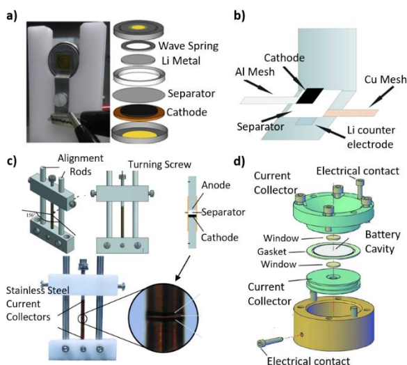
Figure 12. a) A coin cell, along with its schematic representation, mounted on a specially designed holder for the powder diffraction beamline at the Australian Synchrotron. (Reprinted from J. Power Sources, Vol 302, Brant, Li, Gu, and Schmid, Comparative analysis of ex-situ and operando X-ray diffraction experiments for lithium insertion materials, 126-134., Copyright (2016), with permission from Elsevier.) b) Schematic representation of a coffee bag cell before sealing. c) Schematic representation of the cylindrical RATIX cell. d) Schematic representation of the AMPIX cell. Reproduced with permission of the International Union of Crystallography from Refs. 270 [Rosciano, Holzapfel, Kaiser, Scheifele, Ruch, Hahn, Kötz, and Novák, Journal of Synchrotron Radiation (2007)], 268 [Liu, Allan, Borkiewicz, Kurtz, Grey, Chapman, and Chupas, Journal of Applied Crystallography
