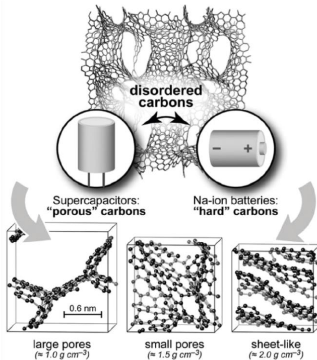
Figure 16. Machine learning approaches for modelling disordered electrodes. Examples of pore structures in disordered carbons, determined from a combination of machine learning and DFT. 286 Different pore sizes are seen experimentally and are each suited to different applications. [V.L. Deringer, C. Merlet, Y. Hu, T.H. Lee, J.A. Kattirtzi, O. Pecher, G. Csányi, S.R. Elliott, and C.P. Grey, Chemical Communications 54, 5988 (2018)] - Published by The Royal Society of Chemistry, reproduced under Creative Commons Attribution CC BY 3.0.
