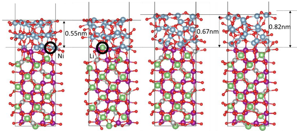
Figure 19. AIRSS search results on the interfacial structure between \text{Al}_2\text{O}_3 and \text{LiNi}_{0.5}\text{Mn}_{1.5}\text{O}_4 .
