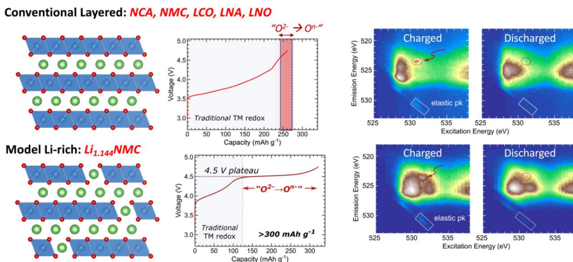
Figure 4. Charge profile and RIXS features observed in the first cycle for a conventional layered transition metal oxide (top) and for a lithium rich layered NMC material (bottom). Adapted from Ref. 62 from The Royal Society of Chemistry under Creative Commons Attribution CC BY 3.0 and with permission from {Z.W. Lebens-Higgins, J. Vinckeviciute, J. Wu, N. V. Faenza, Y. Li, S. Sallis, N. Pereira, Y.S. Meng, G.G. Amatucci, A. Van Der Ven, W. Yang, and L.F.J. Piper, J. Phys. Chem. C 123 , 13201}. Copyright {2019} American Chemical Society.
