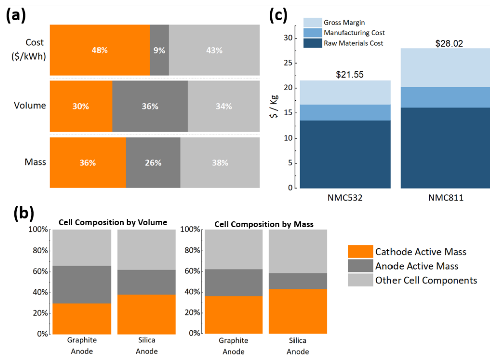
Figure 1. Composition of wet-electrolyte pouch cell. “Other” includes current collectors, separator, electrolyte, binders, cell casing and other minor components of the cell. b) Impact of introducing a high energy density anode on the composition of the cell by volume and mass. c) Cathode active material price and cost structure for NMC532 and NMC811 based on manufacturer reports from China. Source Exawatt (2019 data).
