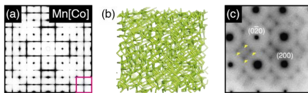
Figure 15. Single-crystal diffuse scattering measurements of disordered cathodes. a) Reconstructed single-crystal diffuse scattering for Mn[Co] Prussian blue analogue in the (hk0) scattering plane; the bottom-right corner is the averaged diffuse scattering pattern in the (hk0) plane. b) Representative pore network for the Mn[Co] Prussian blue analogue in (a), determined from Monte Carlo simulation. 276 c) Experimental electron diffraction pattern of Li 1.2 Mn 0.4 Zr 0.4 O 2 (LMZO) along the zone axis (100). Reproduced from Ref. 277 [Ji, Urban, Kitchaev, Kwon, Artrith, Ophus, Huang, Cai, Shi, Kim, Kim, and Ceder, Nature Communications (2019)] under Creative Commons Attribution CC BY 4.0.
