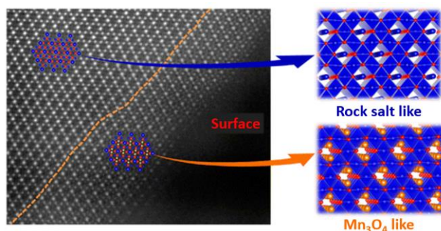
Figure 6. Schematic representation showing the structural complexity of LNMO. HRTEM studies show that during cycling between 3.5 and 4.9 V a Mn 3 O 4 -like phase forms on the surface of LNMO together with a rocksalt-like phase on the subsurface. Reprinted with permission from (M. Lin, L. Ben, Y. Sun, H. Wang, Z. Yang, L. Gu, X. Yu, X.-Q. Yang, H. Zhao, R. Yu, M. Armand, and X. Huang, Chemistry of Materials 27, 292). Copyright (2014) American Chemical Society.
