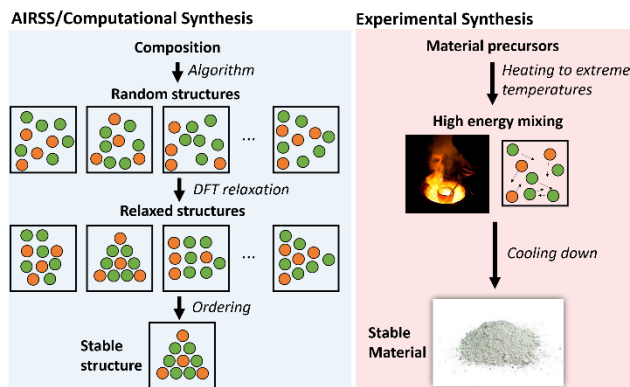
Figure 8. Comparison between an AIRSS search of a composition and an experimental synthesis of a material.
