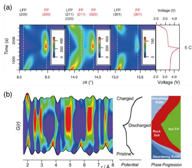
Figure 14. In Situ XRD and operando PDF measurements. a) In situ XRD pattern during fast cycling between LiFePO 4 (LFP) and FePO 4 (FP). The electrochemical reaction proceeds via an intermediate solid solution, which is evident in the diffraction pattern between the LFP and FP states. Dashed lines indicate the peak positions of the LiFePO 4 and FePO 4 phases. 273 From [H. Liu, F.C. Strobridge, O.J. Borkiewicz, K.M. Wiaderek, K.W. Chapman, P.J. Chupas, and C.P. Grey, Science 344, 1252817 (2014).] Reprinted with permission from AAAS. b) Operando PDF data during charge and discharge for an iron oxyfluoride electrode (left); evolution of Fe phases during cycling (right) determined from analysis of operando PDF data. 275 Reprinted with permission from (K.M. Wiaderek, O.J. Borkiewicz, E. Castillo-Martínez, R. Robert, N. Pereira, G.G. Amatucci, C.P. Grey, P.J. Chupas, and K.W. Chapman, Journal of the American Chemical Society 135, 4070). Copyright (2013) American Chemical Society.
