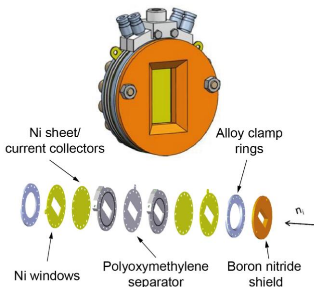
Figure 13. Diagram of an in situ cell used in the POLARIS diffractometer at the ISIS neutron spallation source. Reprinted from Journal of Power Sources, Vol 248, Biendicho, Roberts, Offer, Noréus, Widenkvist, Smith, Svensson, Edström, Norberg, Eriksson, and Hull, New in situ neutron diffraction cell for electrode materials, 900-904., Copyright (2014), with permission from Elsevier.
