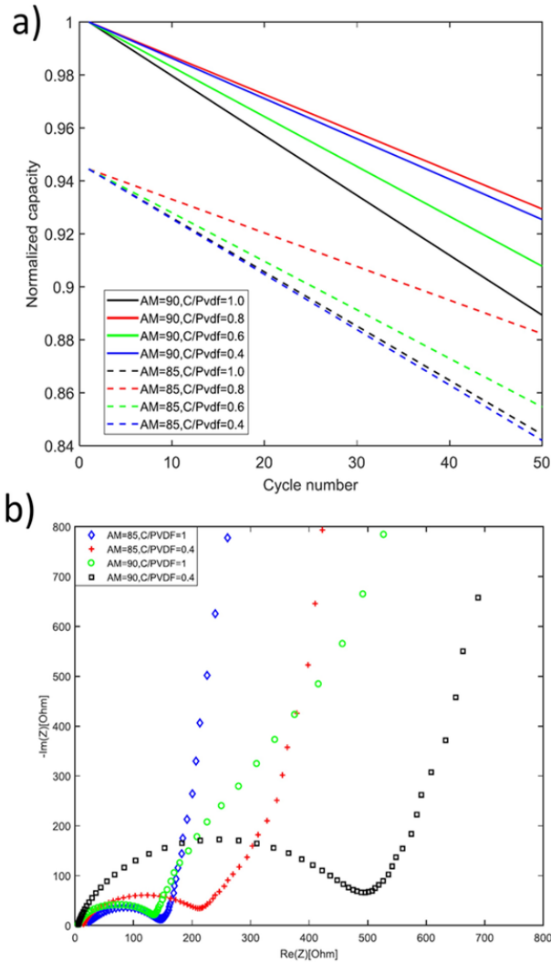
Figure 9. a) Normalized capacity as a function of cycling for \text{LiMn}_2\text{O}_4 and b) EIS spectra with different electrode composition. The electrode composition presents that active material (AM) e.g. 90% for AM=90 and the ratio of conductive material and binder for C/PVDF. Reproduced with permission from MDPI, Basel, Switzerland.
