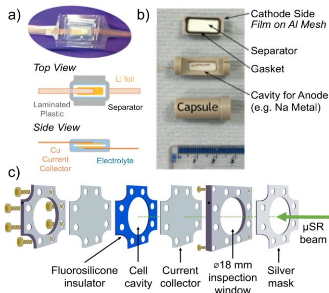
Figure 17. a) NMR bag cell. b) NMR capsule cell. [Adapted from Ref. 295. Copyright 2017 American Chemical Society] under Creative Commons CC BY 4.0 c) \mu SR cell.
