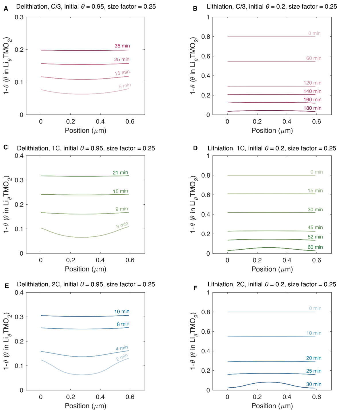
Figure S15. Modelling results showing the spatio-temporal variation of the degree of delithiation at: (A) C/3, (C) 1C, (E) 2C; and lithiation process: (B) C/3, (D) 1C, (F) 2C for a particle size of 600 nm and D_{\text{Li}}^{\text{eff}} = D_{\text{Li}}/3.5 . Lithium occupancies are approximately uniform across the particle for C-rates up to 2C.
