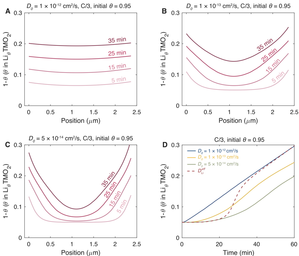
Figure S17. Modelling results showing the spatio-temporal variation of the degree of delithiation at a charge rate of C/3 along the line marked in Figure 3C for different choices of a constant diffusion coefficient D_0 that is independent of the SoC. (A-C) Degree of delithiation within the particle with (A) D_0 = 1 \times 10^{-12} \text{ cm}^2 \text{ s}^{-1} , (B) D_0 = 1 \times 10^{-13} \text{ cm}^2 \text{ s}^{-1} and (C) D_0 = 5 \times 10^{-14} \text{ cm}^2 \text{ s}^{-1} . (D) Corresponding temporal variation of the degree of delithiation at the particle
