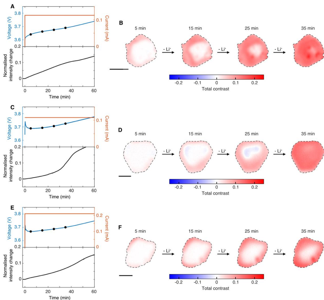
Figure S10. Reproducibility of the lithium heterogeneity at the beginning of charge. Three different particles, from different electrodes and in different cells, are shown here. (A, C, E) Voltage, current and normalised intensity change at a rate of C/3. (B, D, F) Corresponding differential images at the times indicated by black circles. Scale bars, 1 \mu\text{m} .
