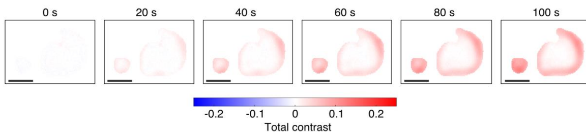
Figure S16. Lithium heterogeneity in particles with different sizes at the beginning of delithiation at 2C. Scale bar, 1 \mu\text{m} .
