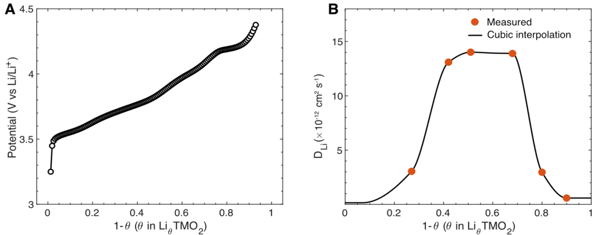
Figure S1. (A) Open circuit voltage ( V_{\text{oc}} ) measured at different states of charge in the GITT experiment. (B) The ab - plane diffusivity obtained from the \text{Li}^+ hop rate. The NMR data is shown as discrete data points and a smooth curve using piecewise cubic interpolation functions is fitted to this data for use in the numerical simulations.
