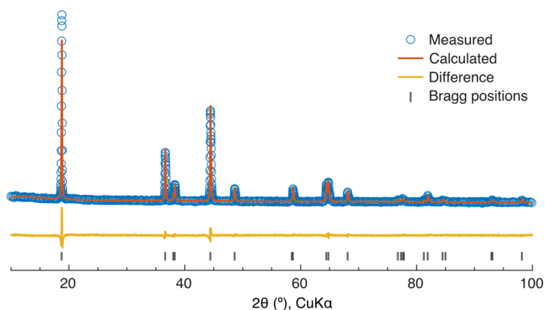
Figure S5. X-ray diffraction pattern and Rietveld refinement results. Lattice constants: a = 2.87551(7) \text{ \AA} , c = 14.1944(5) \text{ \AA} ; unit cell volume: 101.643(6) \text{ \AA}^3 . Li/Ni paired antisite defects: 2.0%. Fitting quality: R_{wp} = 3.43\% , R_{exp} = 1.50\% , gof = 2.28 .
