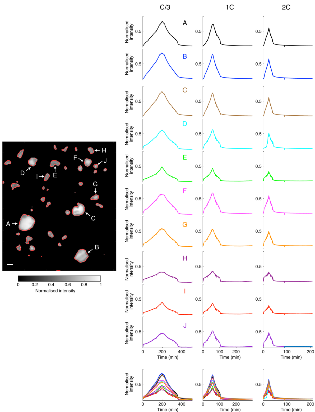
Figure S11. Normalised intensity changes for multiple particles within the same electrode at various rates (C/3, 1C and 2C).
