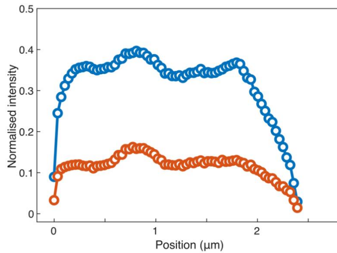
Figure S18. Line plots of the normalised intensity as a function of position at the end of CC discharge at 1C rate (blue) and after an additional two-hours voltage hold at 3 V (red).
