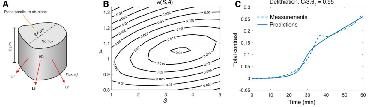
Figure S2. (A) Schematic of the NMC particle used in the simulation. (B) Contour plot of the error function e(S, A) for the C/3 delithiation experiment. The global minimum of error is attained at (S, A) = (3.5, 1/0.95) . (C) Comparison between measurements and predictions of the total contrast at the center of the particle in the C/3 delithiation experiment with (S, A) = (3.5, 1/0.95) .
