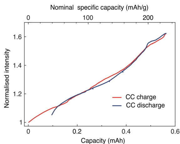
Figure S8. Normalised intensity change as a function of capacity during a C/3 CC-CC charge-discharge cycle. The nominal specific capacity is normalised to the mass of the NMC active material.
