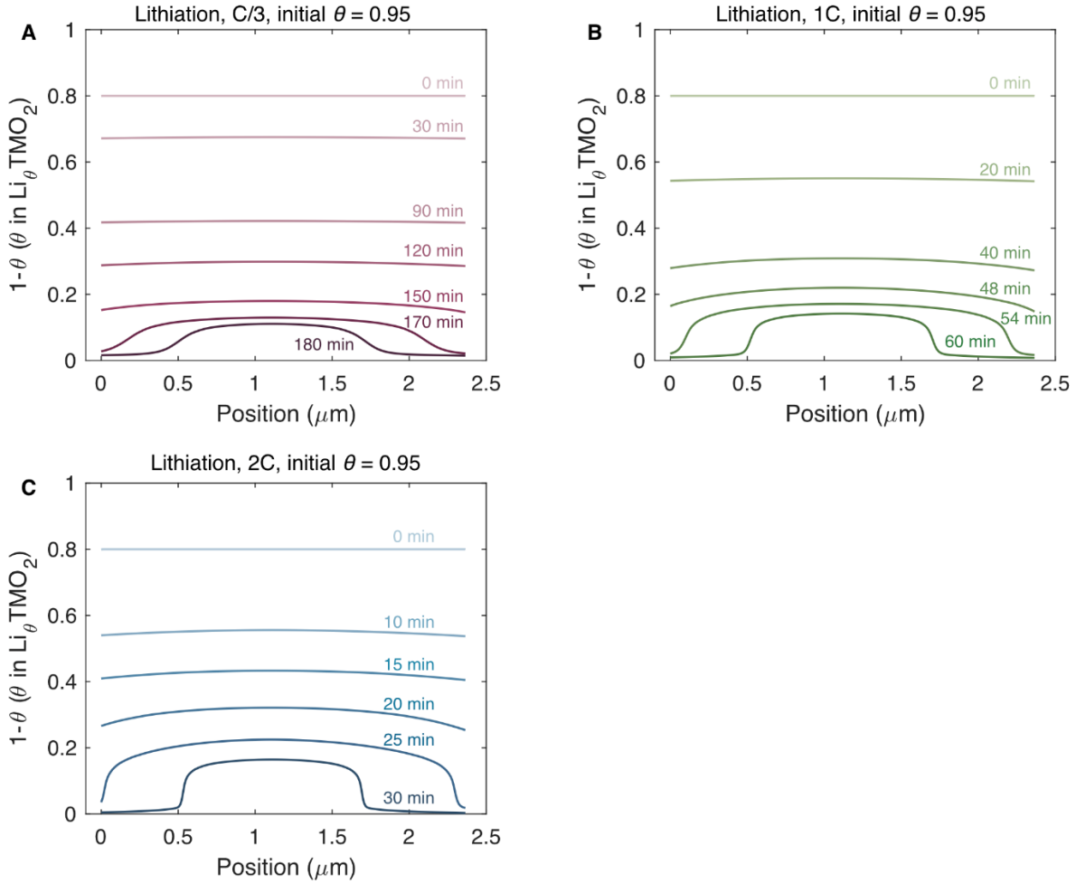
Figure S19 Modelling results showing the spatio-temporal variation of the degree of delithiation at (A) C/3, (B) 1C and (C) 2C, along the horizontal line marked in Figure 3C with D_{\text{Li}}^{\text{eff}} = D_{\text{Li}}/3.5 . Significant lithium heterogeneities are observed when the occupancy in the particle exceeds \theta = 0.8 ( 1 - \theta = 0.2 ), caused by a drop in the diffusivity to the order of 10^{-12} \text{cm}^2 \text{s}^{-1} . The occupancy at the particle centre lags significantly behind the surface near the end of lithiation for all three C-rates, with 2C showing the largest gradient across the particle.
