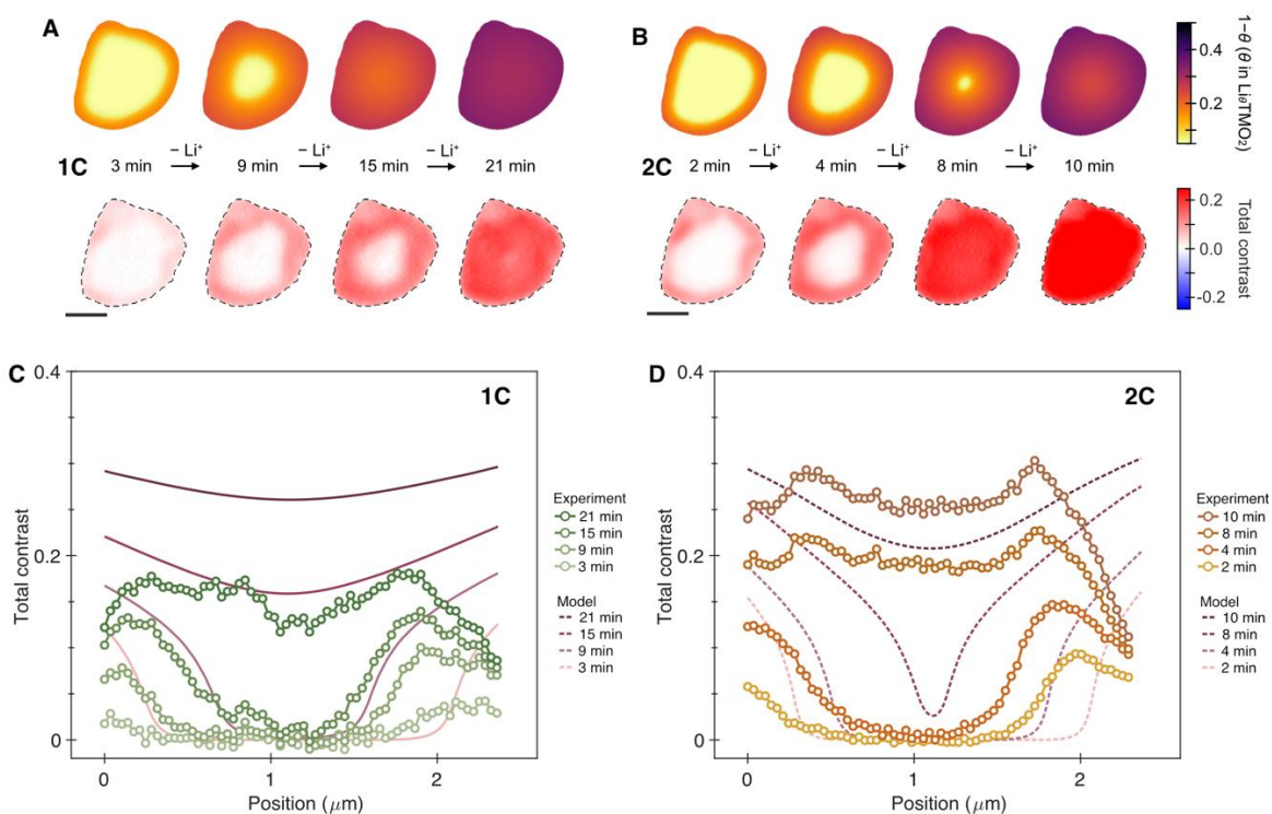
Figure S13. Modelling and experimental results of delithiation 1C ( A, C ) and 2C rates ( B, D ), where the model used D_{\text{Li}}^{\text{eff}} \equiv D_{\text{Li}}/3.5 .
