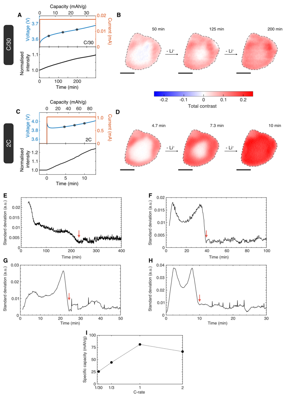
Figure S12. Rate response. ( A , B ) Voltage, current and normalised intensity change ( A ) and the representative differential images ( B ) at a rate of C/30. ( C , D ) Voltage, current and normalised intensity change ( C ) and the representative differential images ( D ) at a rate of 2C. ( E - H ) The evolution of the standard deviation of the ‘sequential differential contrast’ over the imaged particle pixels for C/30 ( E ), C/3 ( F ), 1C ( G ) and 2C ( H ). ‘Sequential differential contrast’ = (I_k - I_{(k-x)})/I_{(k-x)} , where I_k is the intensity of the k^{\text{th}} frame and I_{(k-x)} is the intensity of the (k-x)^{\text{th}} frame, which represents intensity changes occurring in the time interval between the pair of frames ( x , 20 for C/30, 30 for C/3, 1C and 2C. Note for the C/30 dataset, every 20 frames were binned to improve statistics). Red arrows indicate a sharp drop in standard deviation which occurs when the propagating delithiation front reaches the centre of the particle, marking the disappearance of the
