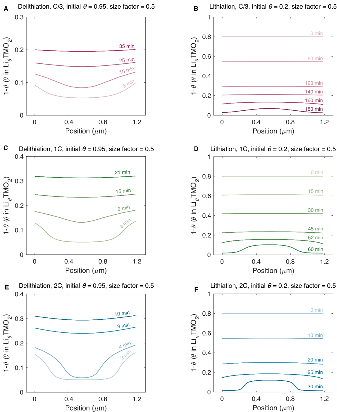
Figure S14. Modelling results showing the spatio-temporal variation of the degree of delithiation at: (A) C/3, (C) 1C, (E) 2C; and lithiation process: (B) C/3, (D) 1C, (F) 2C for a particle size of 1.2 \mu\text{m} and D_{\text{Li}}^{\text{eff}} = D_{\text{Li}}/3.5 . Lithium heterogeneity is significantly reduced at low C-rate of C/3 when compared to the original particle Figure 3D .
