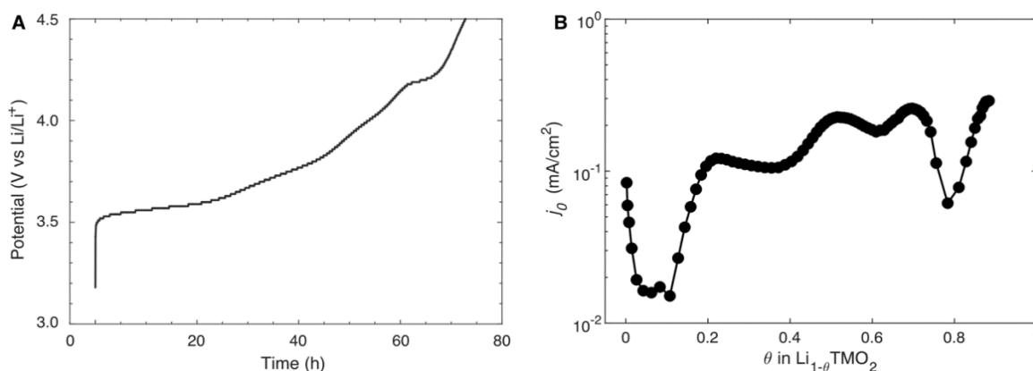
Figure S20. Potentiostatic intermittent titration technique (PITT) results. (A) Voltage profile obtained from PITT experiment. (B) Exchange current density as a function of SoC.
