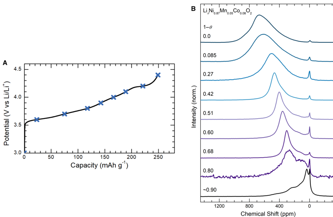
Figure S3. ^7\text{Li} MATPASS spectra measured from \text{Li}_\theta\text{Ni}_{0.87}\text{Mn}_{0.05}\text{Co}_{0.08}\text{O}_2 at various values of 1-\theta , as indicated on the figure. Intensities are normalised to the most intense peak. MAS, 60 kHz.
